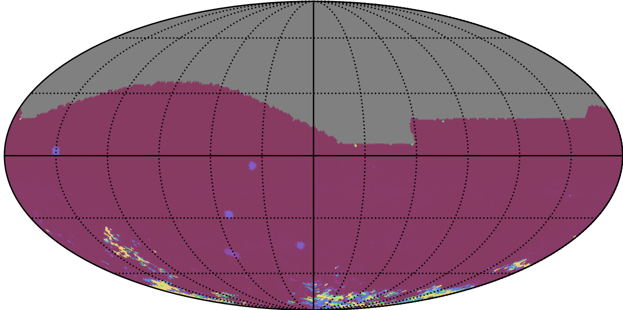
ddf_acor_sf15_lsf30_lsr50_v3.4_10yrs All sky iz bands: 75th Percentile Intranight Timespan
