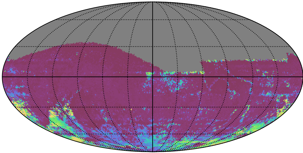
ddf_acor_sf15_lsf30_lsr50_v3.4_10yrs All sky i band: 75th Percentile Intranight Timespan
