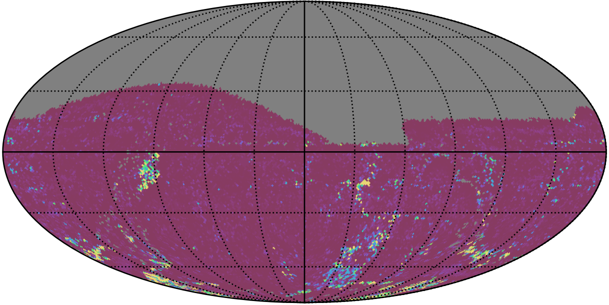
ddf_acor_sf15_lsf30_lsr50_v3.4_10yrs All sky g band: 75th Percentile Intranight Timespan
