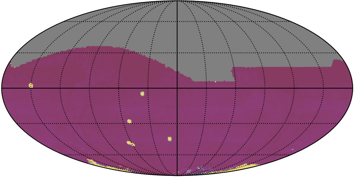
ddf_acor_sf15_lsf30_lsr50_v3.4_10yrs All sky all bands: 75th Percentile Intranight Timespan
