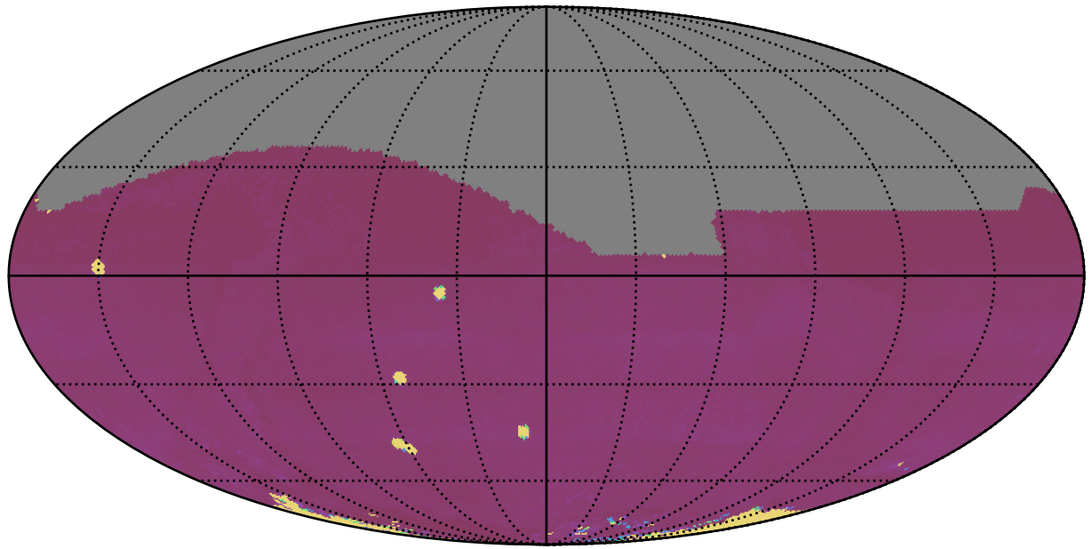
ddf_acor_sf15_lsf30_lsr50_v3.4_10yrs All sky: 75th Percentile Intranight Timespan
