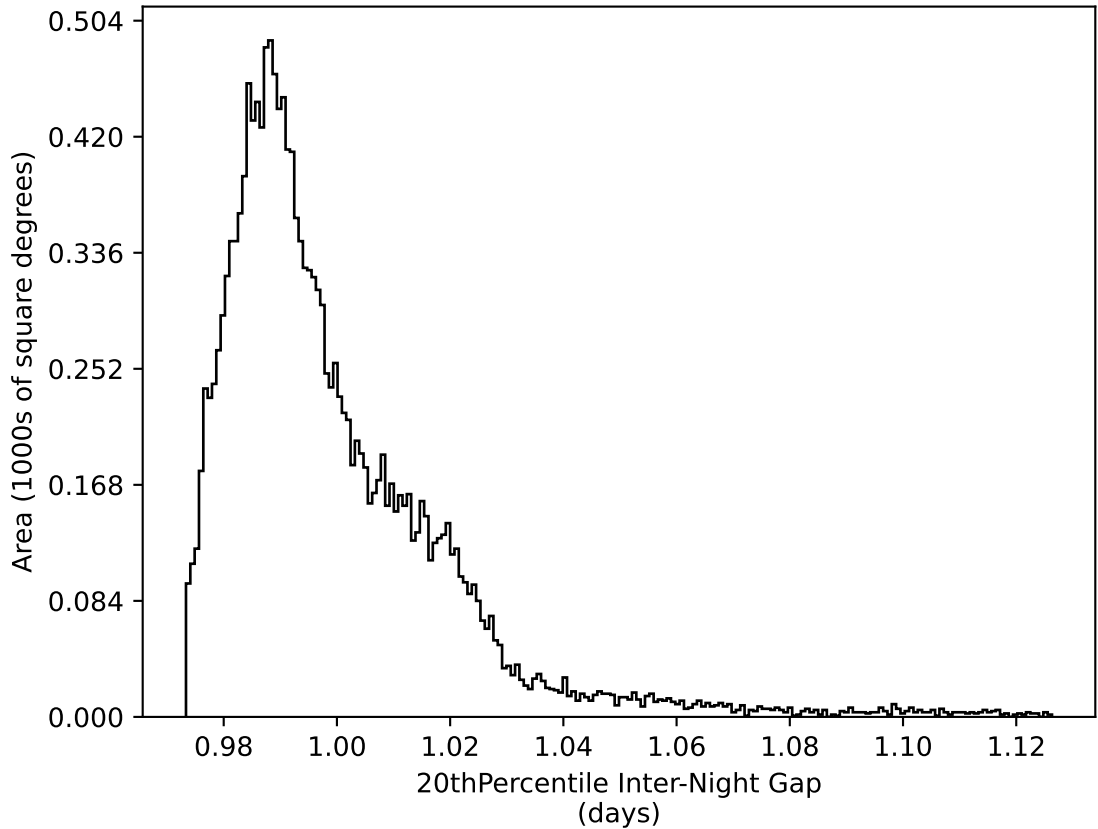
ddf_acor_sf15_ls30_lsr50_v3.4_10yrs WFD all bands: 20thPercentile Inter-Night Gap
