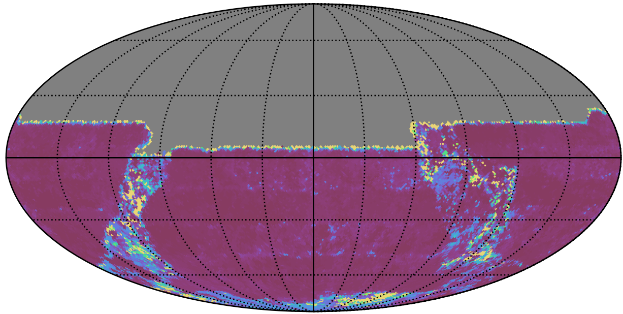
ddf_acor_sf15_lsf30_lsr50_v3.4_10yrs All sky u band: 20thPercentile Inter-Night Gap
