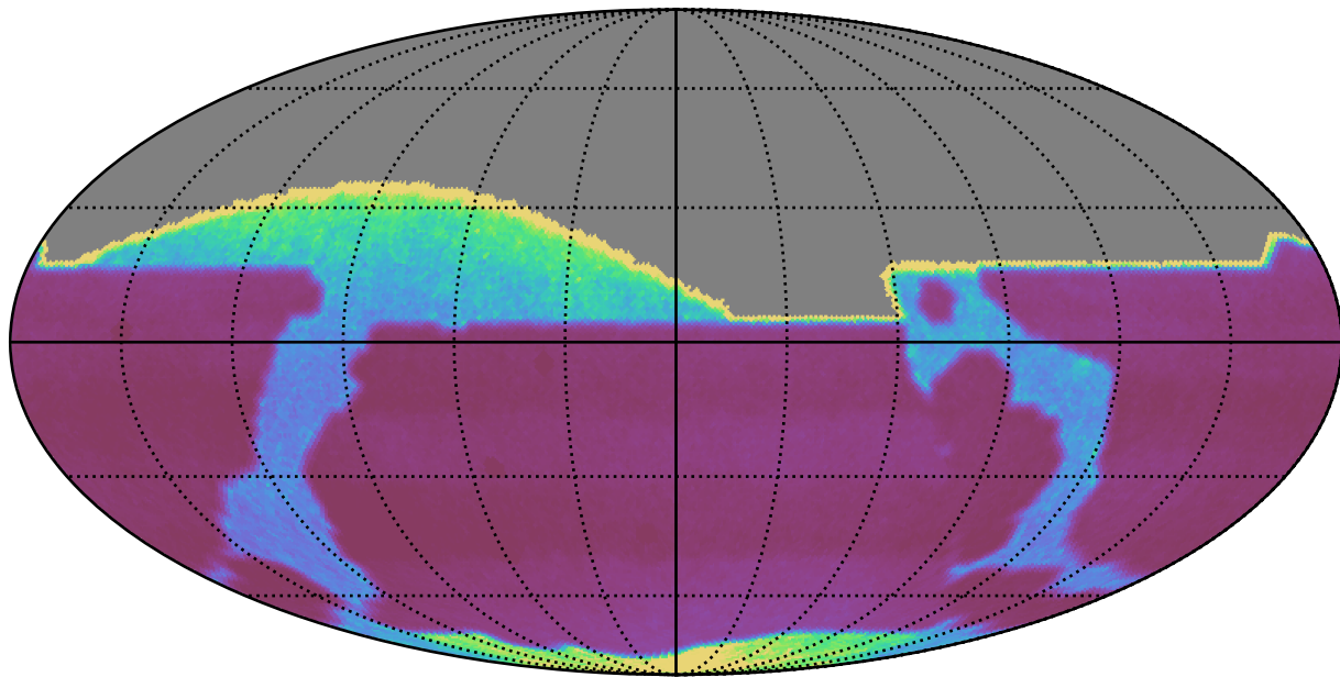
ddf_acor_sf15_lsf30_lsr50_v3.4_10yrs : properMotion
