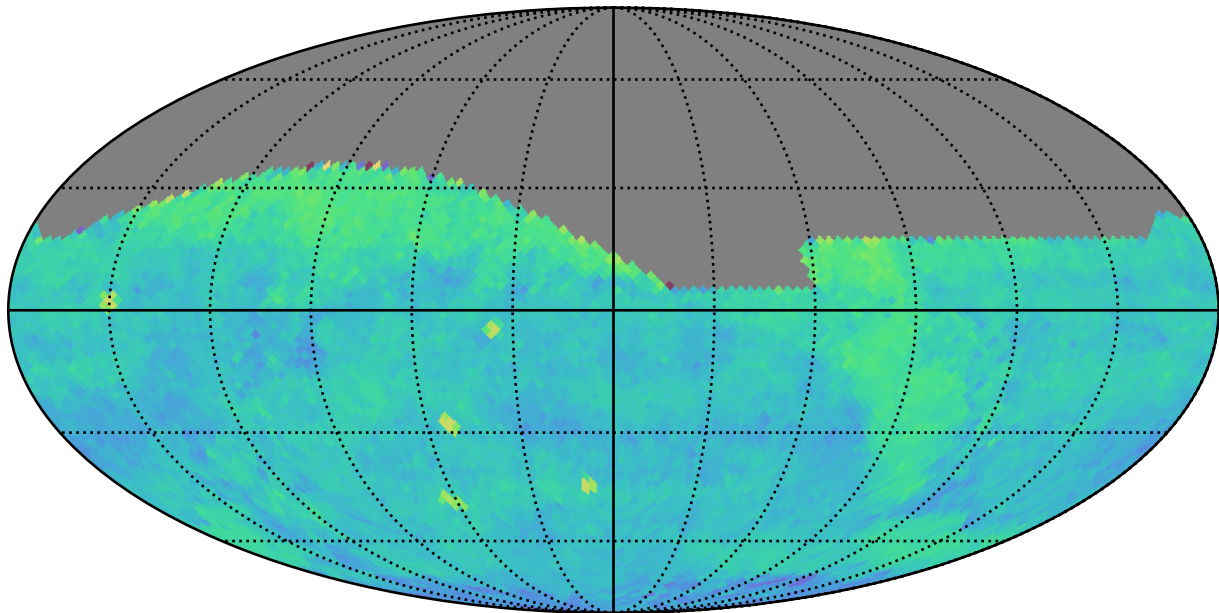
ddf_acor_sf15_lsf30_lsr50_v3.4_10yrs (g or r or i): PairFraction
