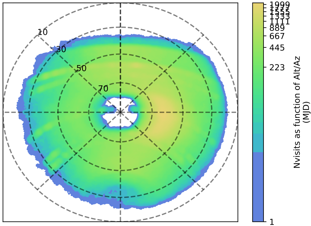
ddf_acor_sf15_lsf30_lsr50_v3.4_10yrs y: Nvisits as function of Alt/Az
