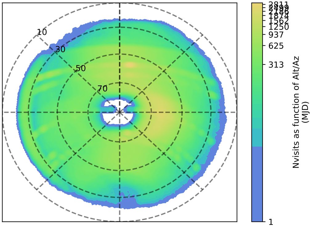
ddf_acor_sf15_ls30_lsr50_v3.4_10yrs r: Nvisits as function of Alt/Az
