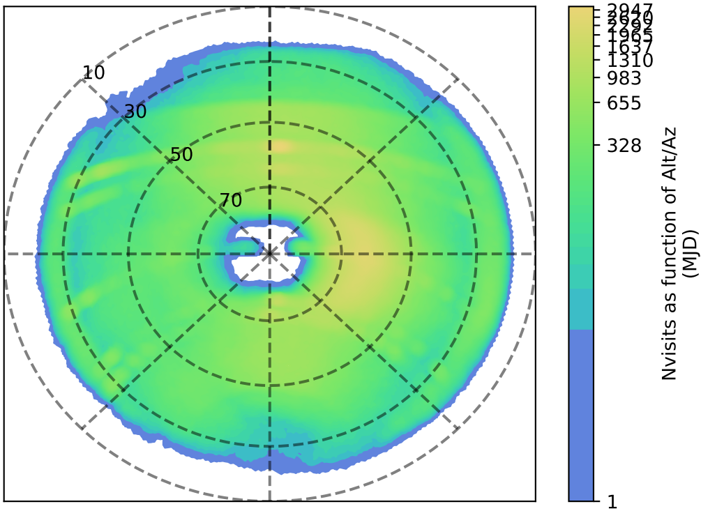
ddf_acor_sf15_ls30_lsr50_v3.4_10yrs i: Nvisits as function of Alt/Az
