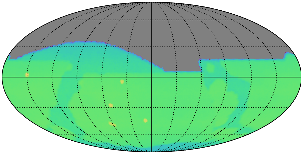
ddf_acor_sf15_lsf30_lsr50_v3.4_10yrs : CoaddM5
