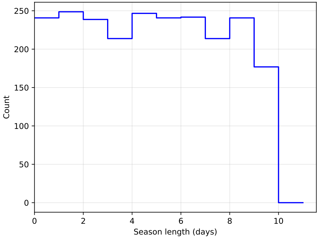
ddf_acor_sf15_lsf30_lsr50_v3.4_10yrs DD:ECDFS all bands: SeasonLength
