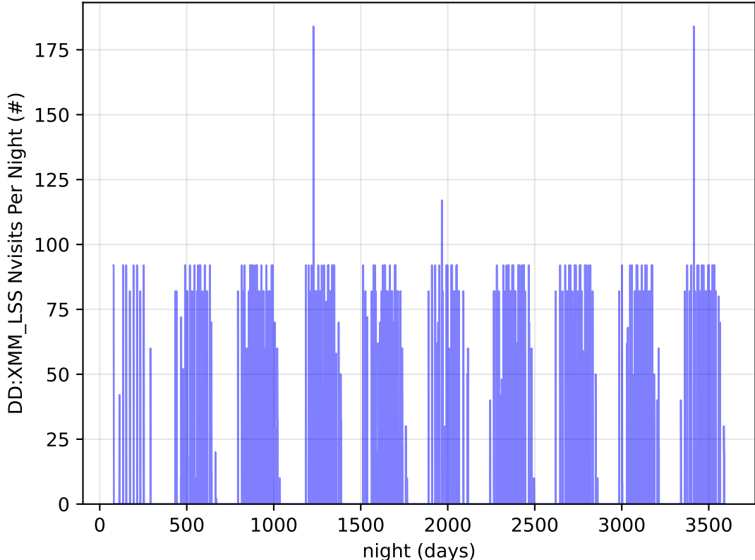
ddf_acor_sf15_lsf30_lsr50_v3.4_10yrs all bands: DD:XMM_LSS Nvisits Per Night
