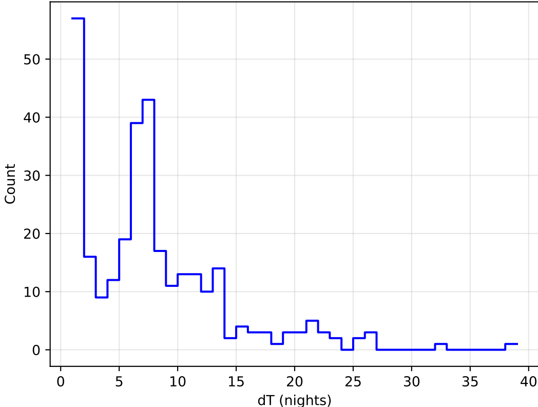
ddf_acor_sf15_lsf30_lsr50_v3.4_10yrs all bands: DD:XMM_LSS Delta Nights Histogram
