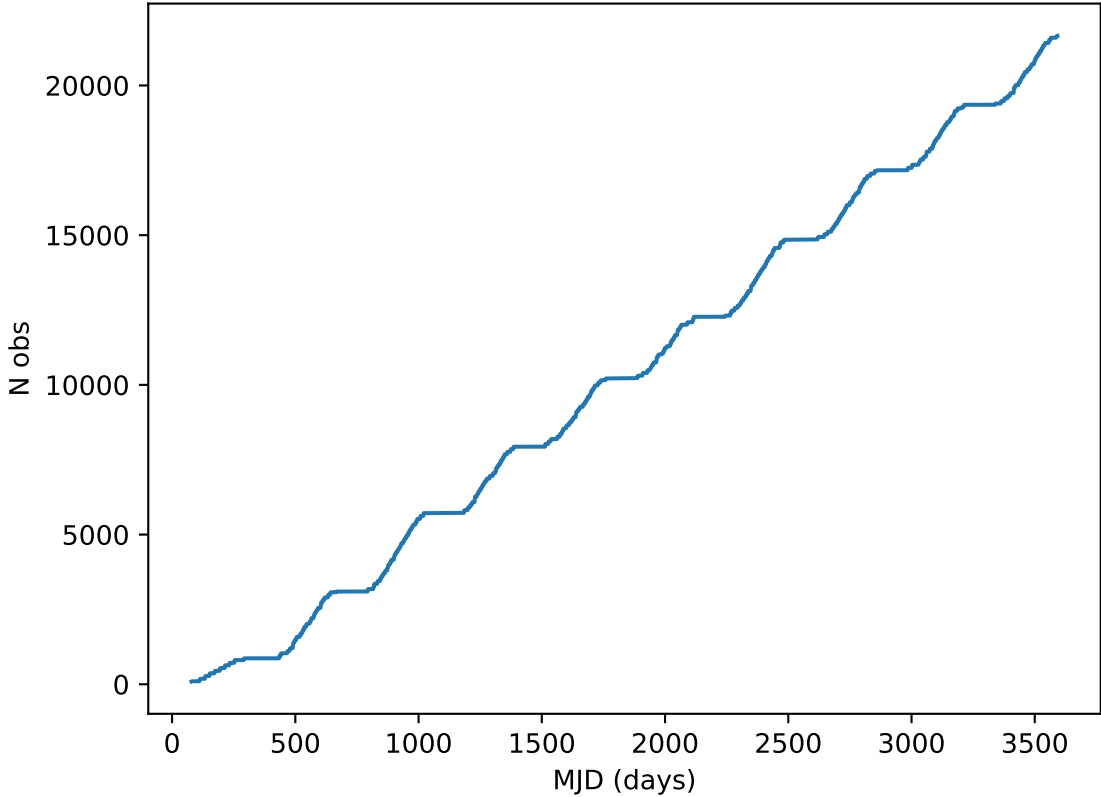
ddf_acor_sf15_lsf30_lsr50_v3.4_10yrs all bands: DD:XMM_LSS Cumulative NVisits
