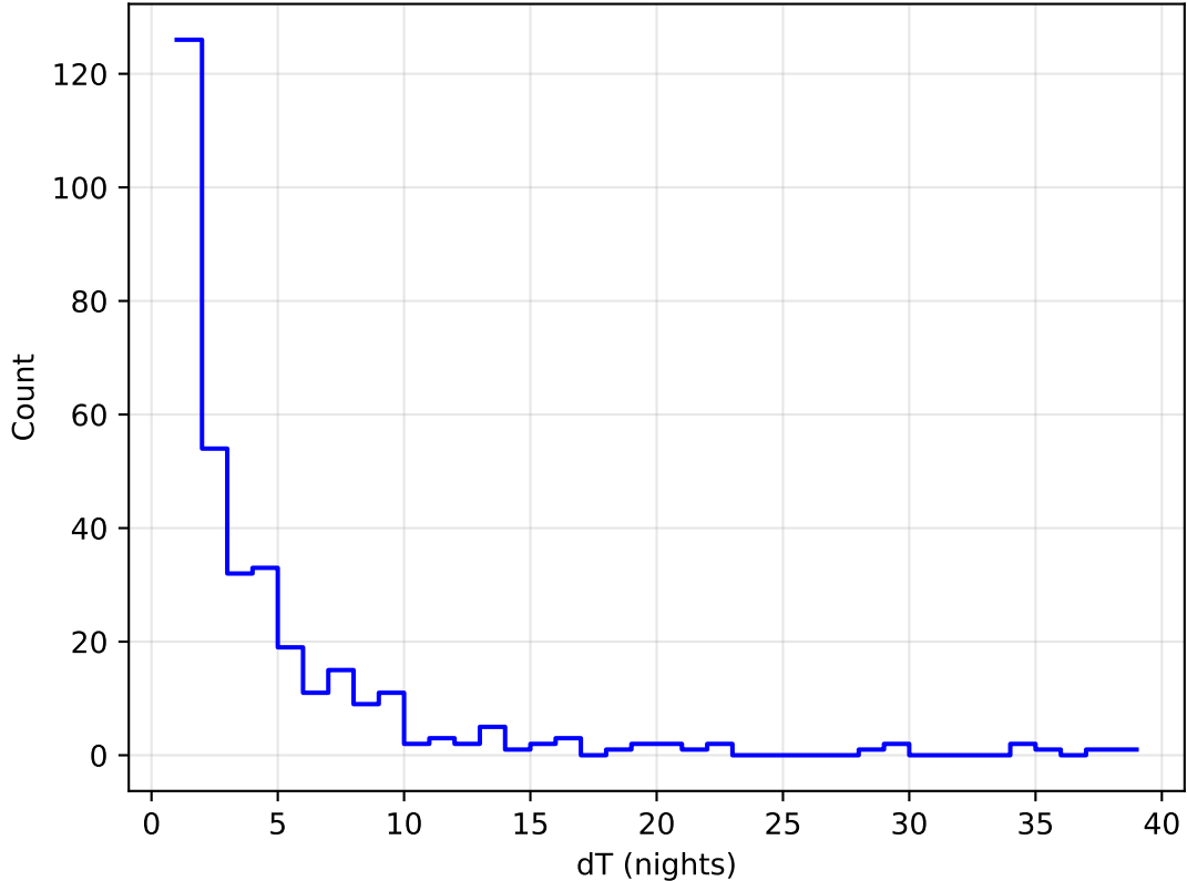
ddf_acor_sf15_lsf30_lsr50_v3.4_10yrs all bands: DD:WFD Delta Nights Histogram
