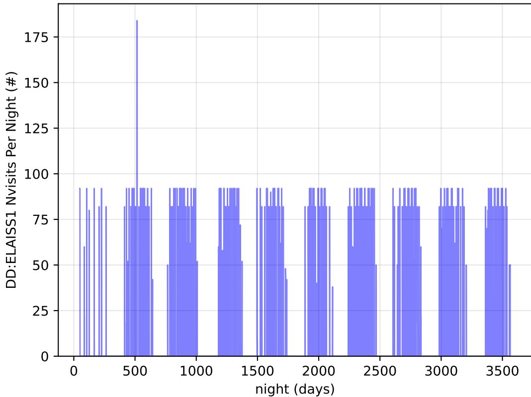
ddf_acor_sf15_lsf30_lsr50_v3.4_10yrs all bands: DD:ELAISS1 Nvisits Per Night
