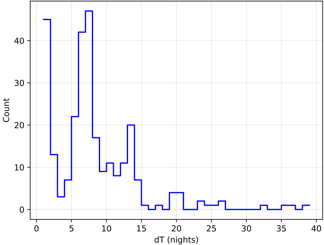
ddf_acor_sf15_lsf30_lsr50_v3.4_10yrs all bands: DD:ELAISS1 Delta Nights Histogram
