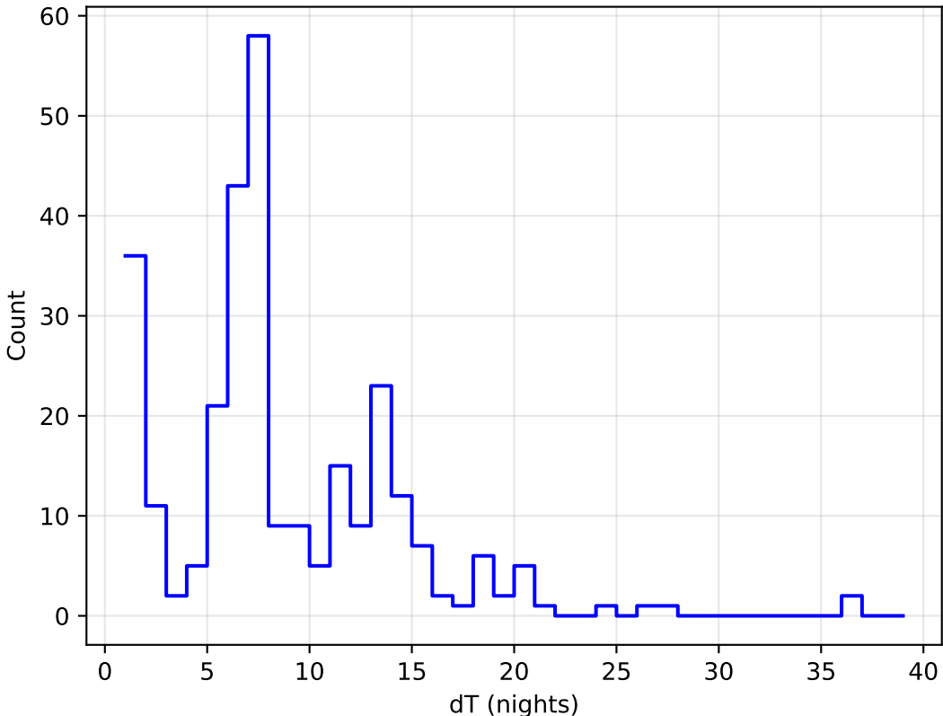
ddf_acor_sf15_lsf30_lsr50_v3.4_10yrs all bands: DD:EDFS Delta Nights Histogram
