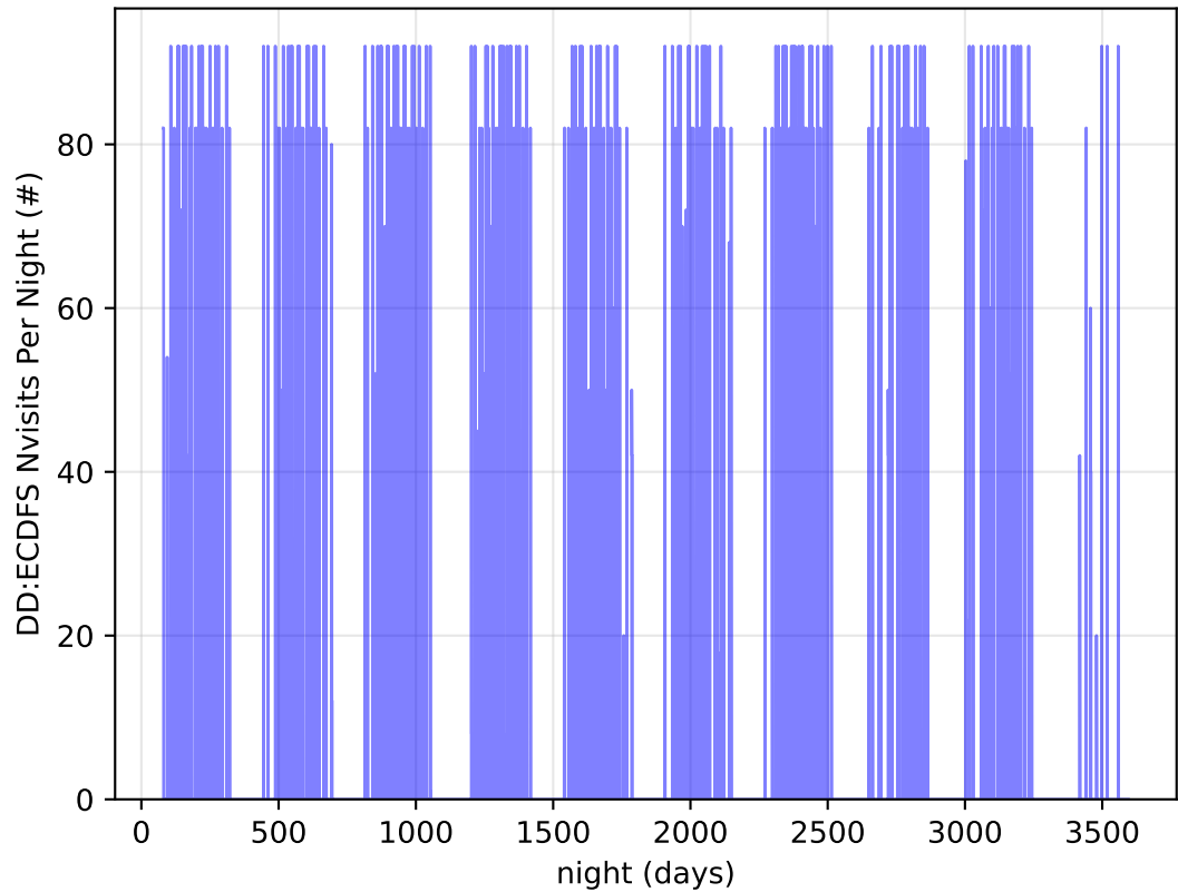
ddf_acor_sf15_lsf30_lsr50_v3.4_10yrs all bands: DD:ECDFS Nvisits Per Night
