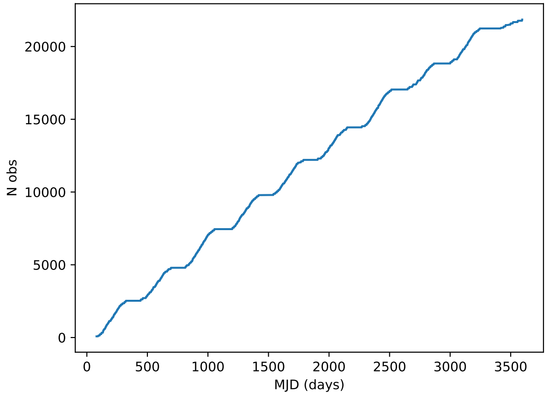
ddf_acor_sf15_lsf30_lsr50_v3.4_10yrs all bands: DD:ECDFS Cumulative NVisits
