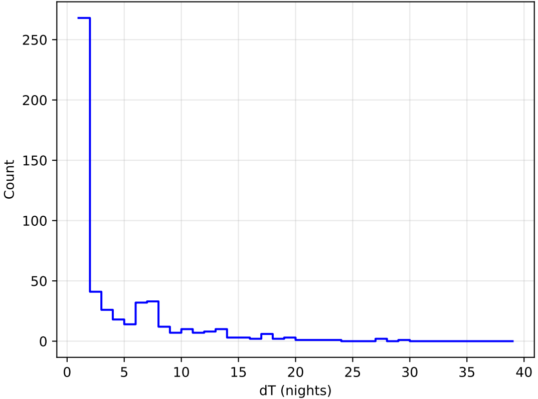
ddf_acor_sf15_Isf30_Isr50_v3.4_10yrs all bands: DD: COSMOS Delta Nights Histogram
