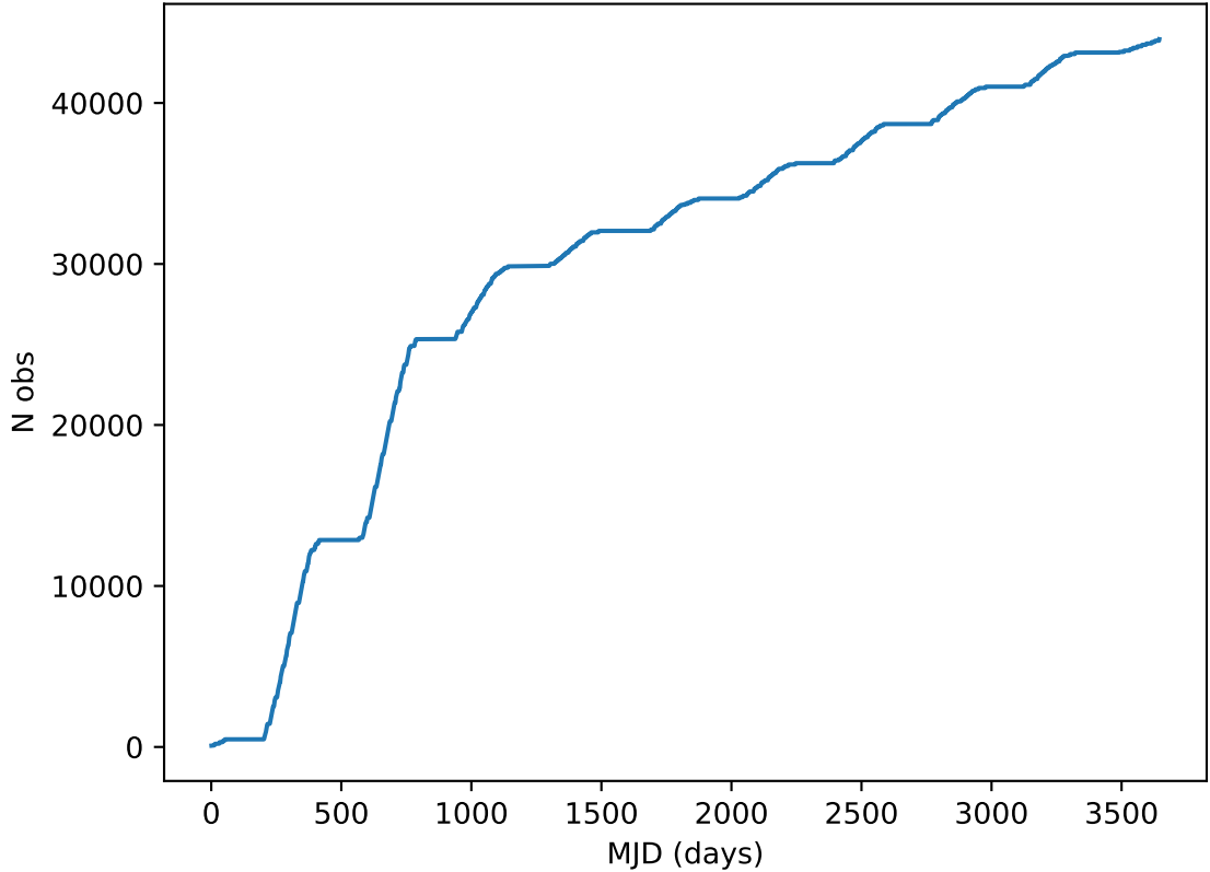
ddf_acor_sf15_lsf30_lsr50_v3.4_10yrs all bands: DD: COSMOS Cumulative NVisits
