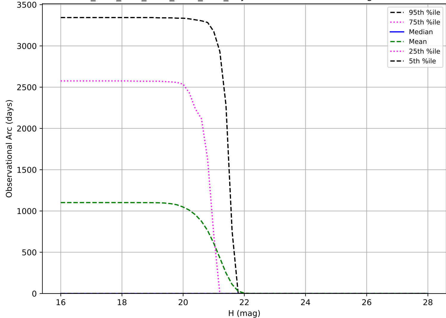
ddf_acor_sf15_lsf30_lsr20_v3.4_10yrs: Observational Arc Length Vatira
