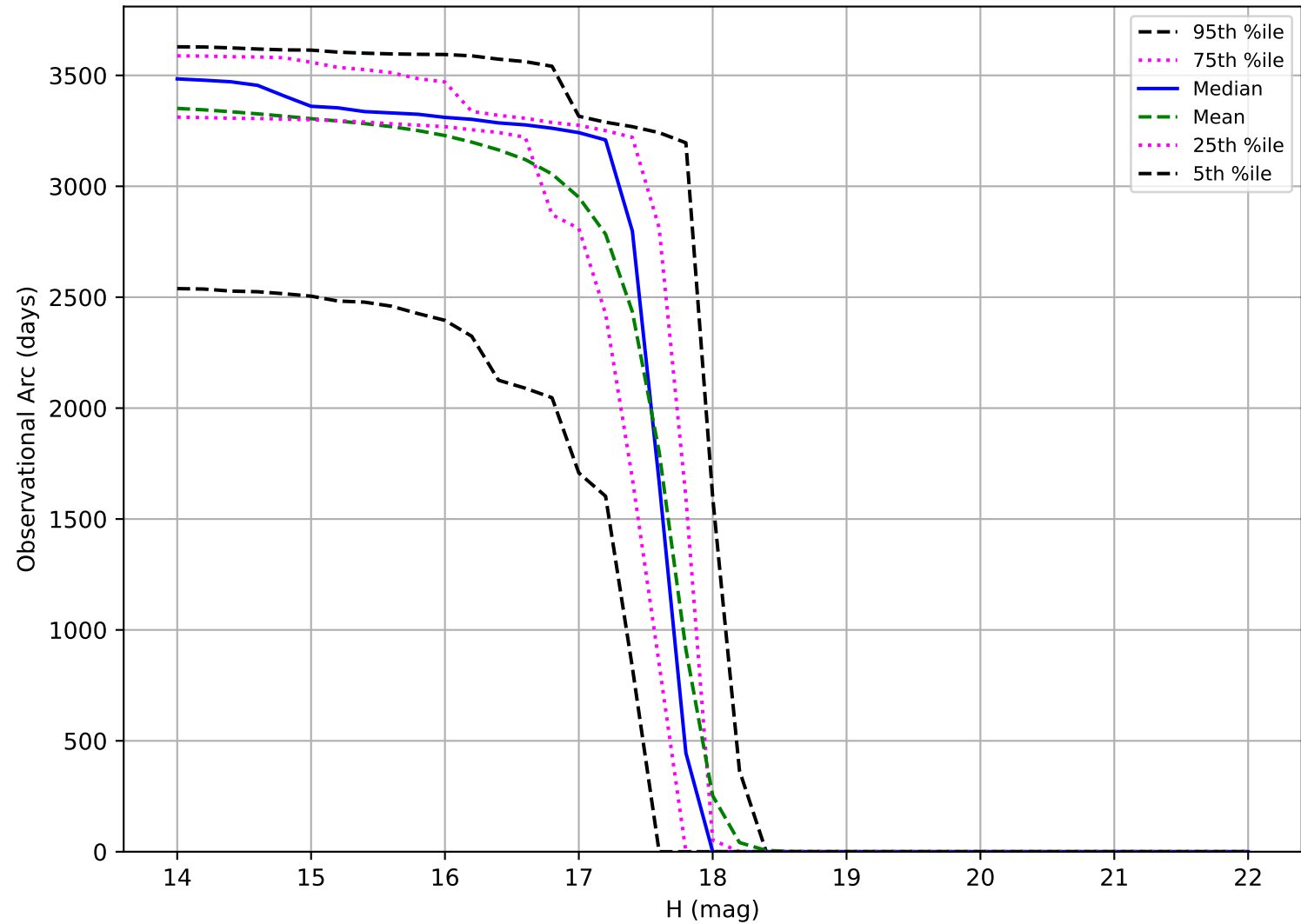
ddf_acor_sf15_lsf30_lsr20_v3.4_10yrs: Observational Arc Length Trojan
