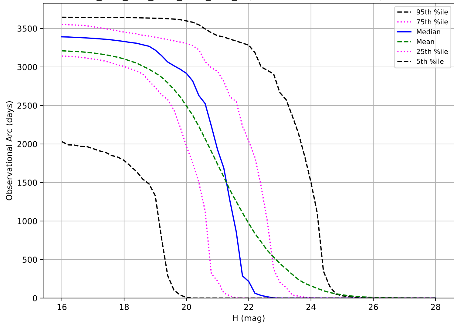
ddf_acor_sf15_lsf30_lsr20_v3.4_10yrs: Observational Arc Length PHA
