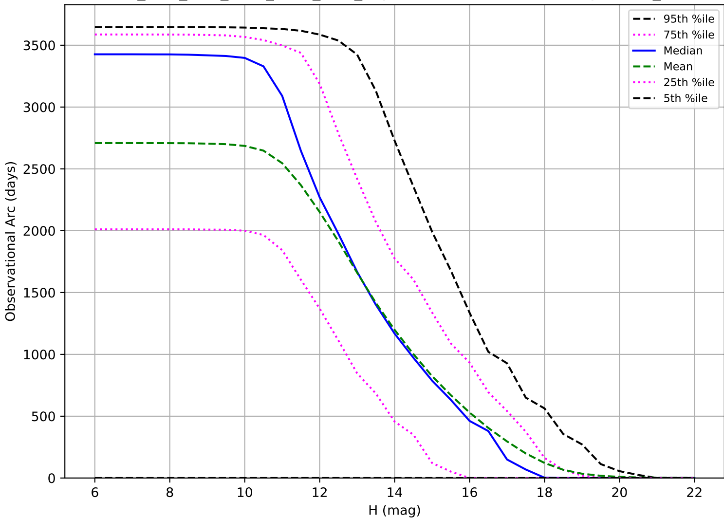
ddf_acor_sf15_lsf30_lsr20_v3.4_10yrs: Observational Arc Length OCC_r5
