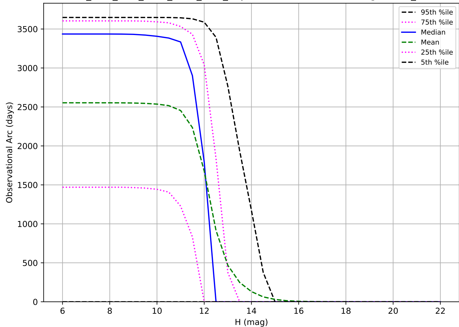
ddf_acor_sf15_lsf30_lsr20_v3.4_10yrs: Observational Arc Length OCC_r20
