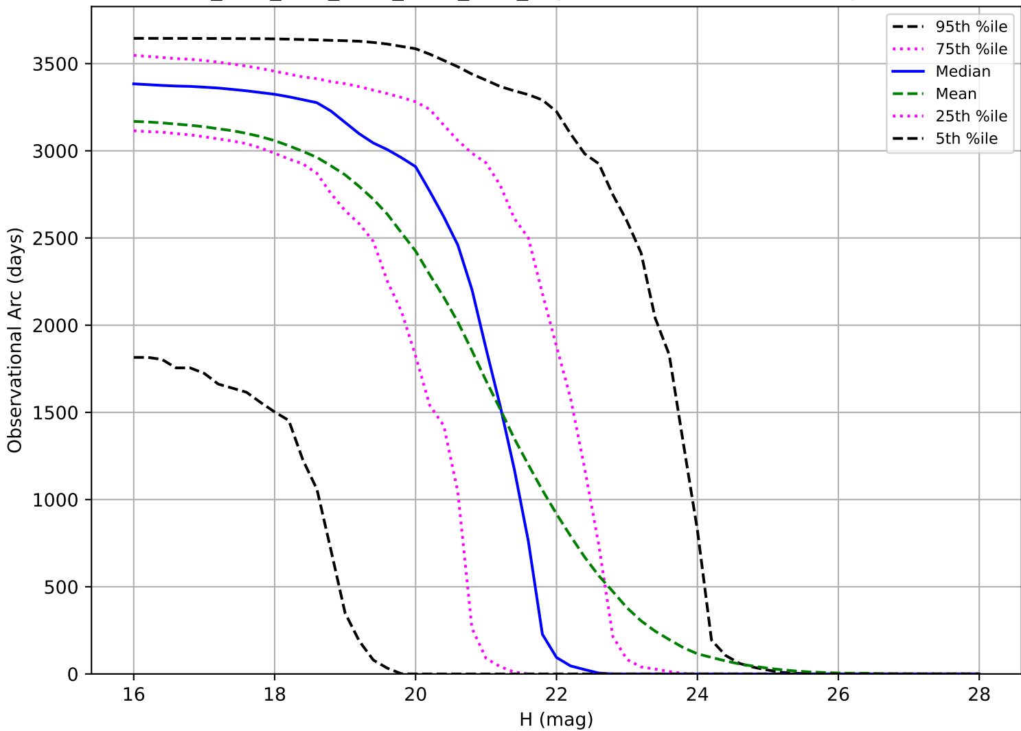
ddf_acor_sf15_lsf30_lsr20_v3.4_10yrs: Observational Arc Length NEO
