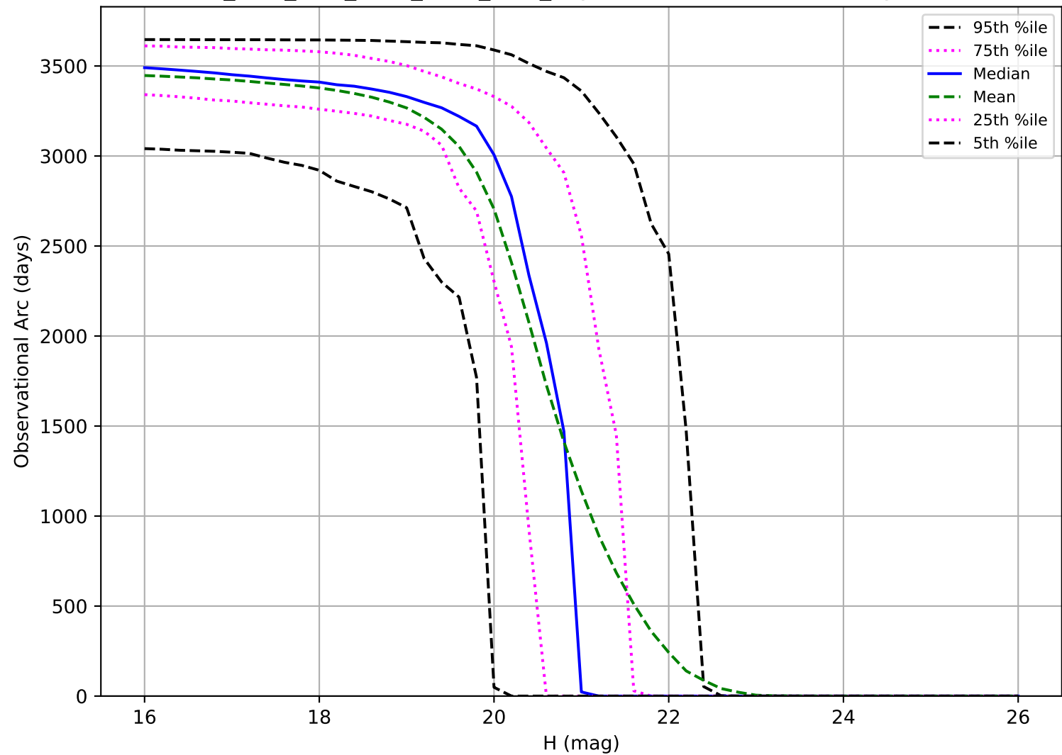
ddf_acor_sf15_lsf30_lsr20_v3.4_10yrs: Observational Arc Length MBA
