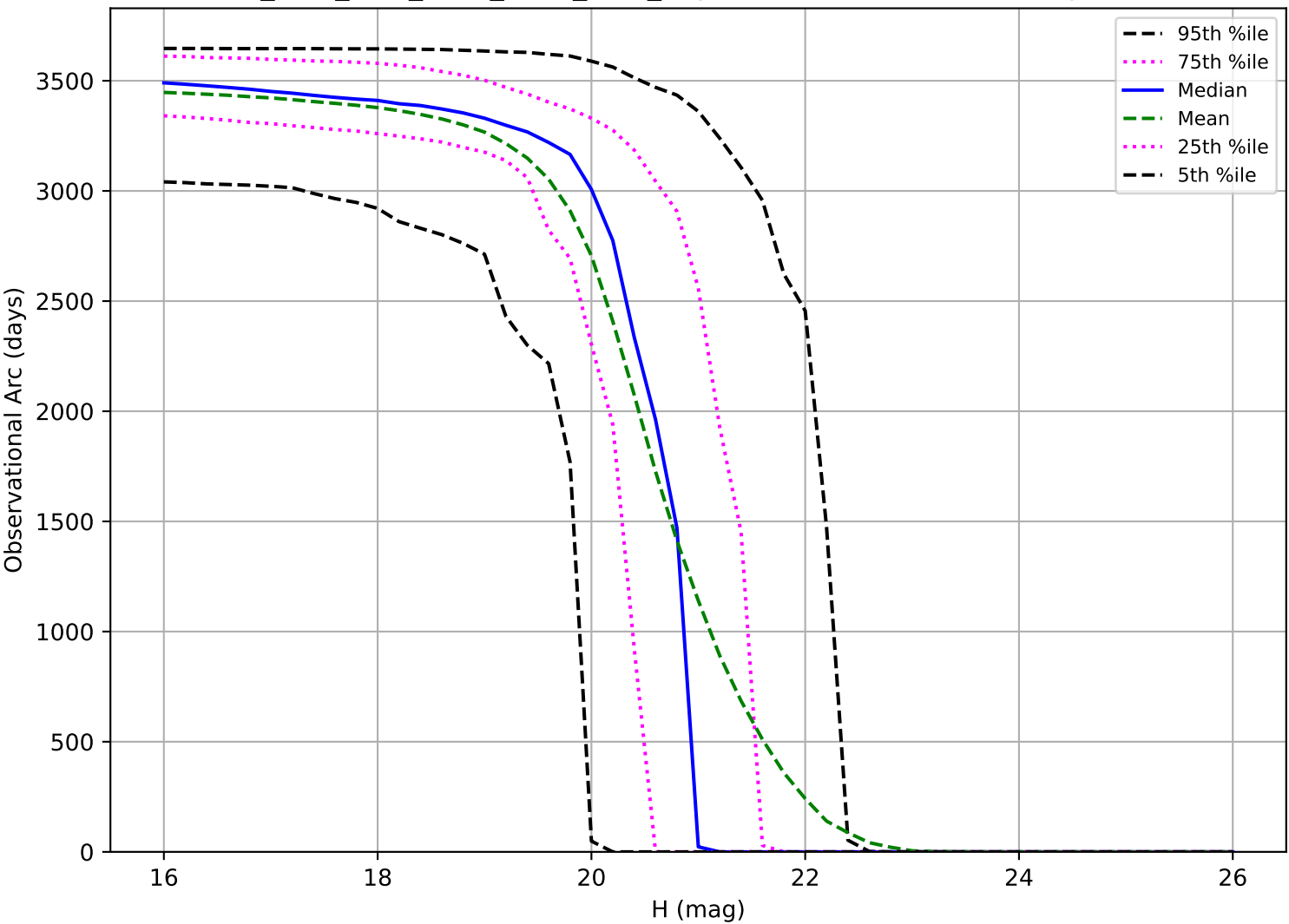
ddf_acor_sf15_lsf30_lsr20_v3.4_10yrs: Observational Arc Length MBA
