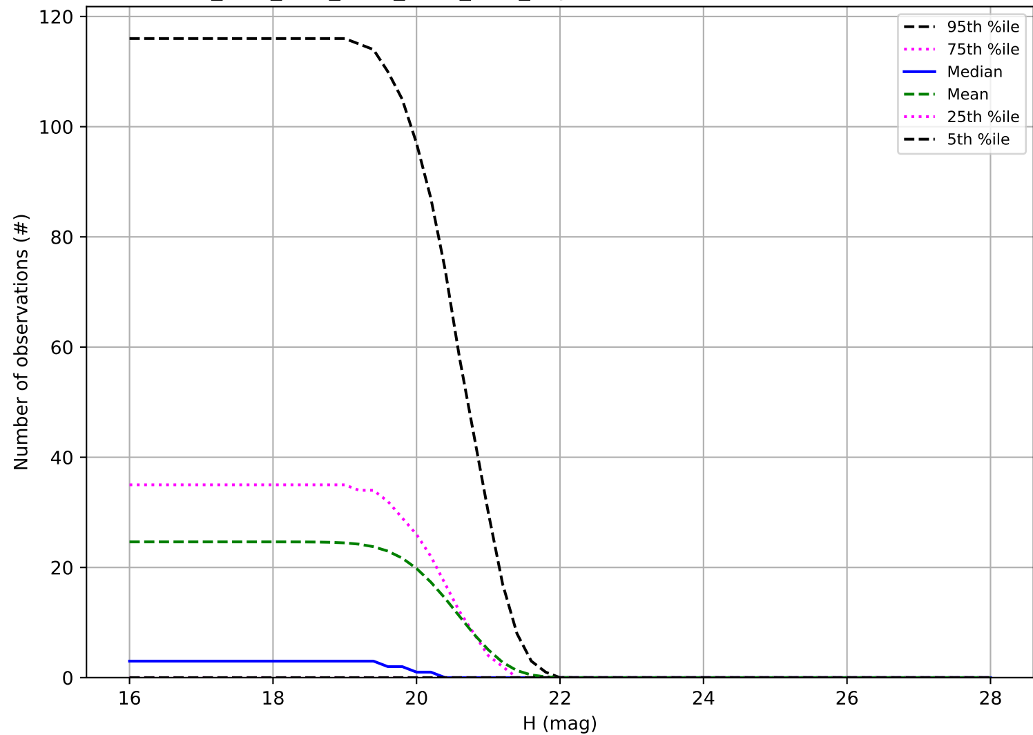
ddf_acor_sf15_lsf30_lsr20_v3.4_10yrs: Number of observations Vatira
