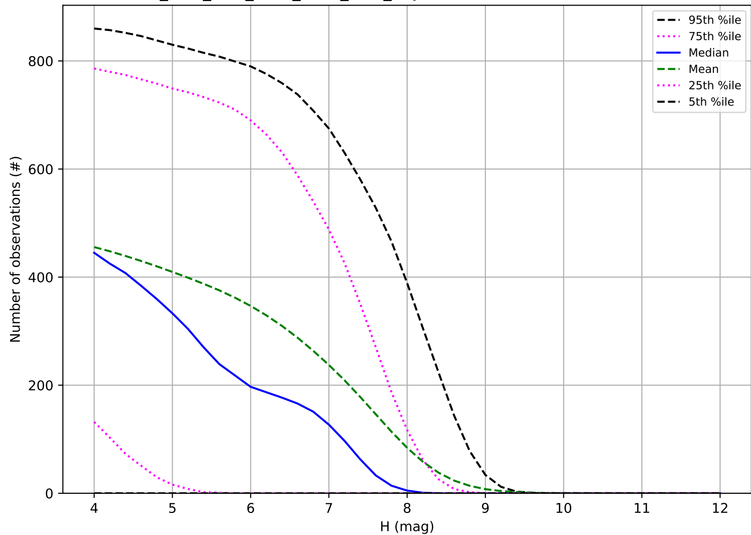
ddf_acor_sf15_lsf30_lsr20_v3.4_10yrs: Number of observations TNO
