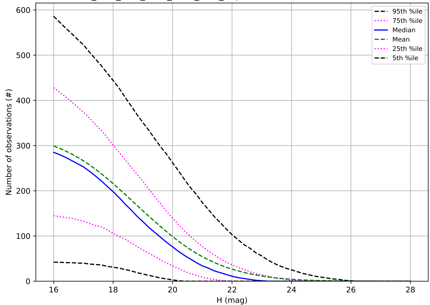
ddf_acor_sf15_lsf30_lsr20_v3.4_10yrs: Number of observations PHA
