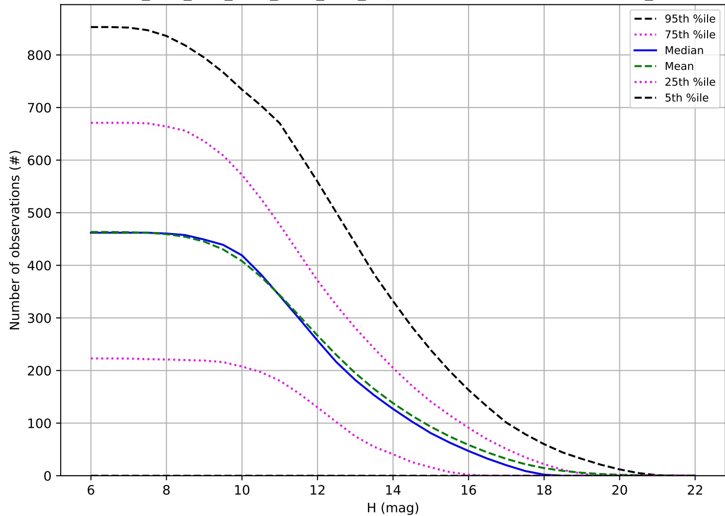
ddf_acor_sf15_lsf30_lsr20_v3.4_10yrs: Number of observations OCC_r5
