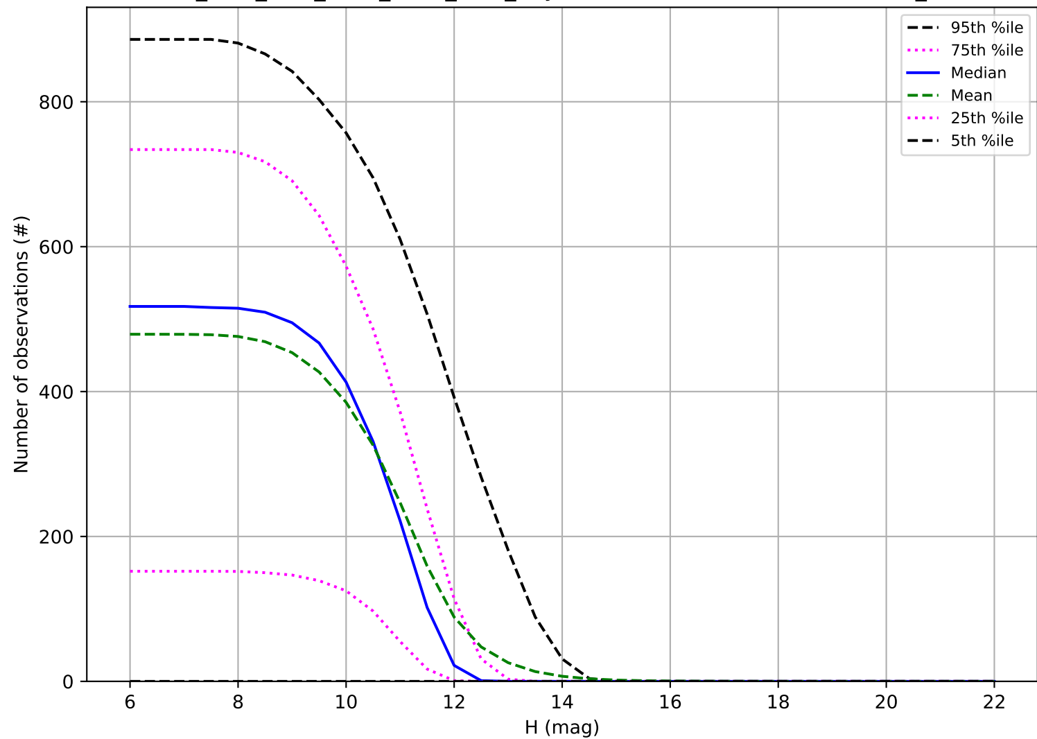
ddf_acor_sf15_lsf30_lsr20_v3.4_10yrs: Number of observations OCC_r20
