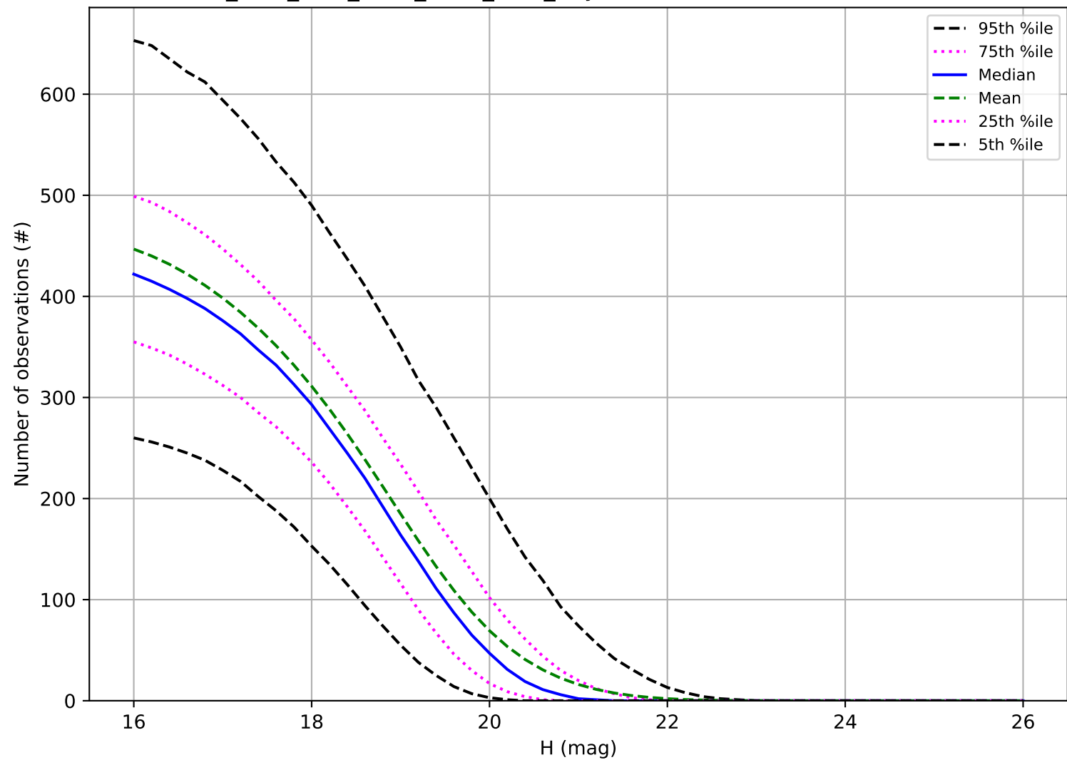
ddf_acor_sf15_lsf30_lsr20_v3.4_10yrs: Number of observations MBA
