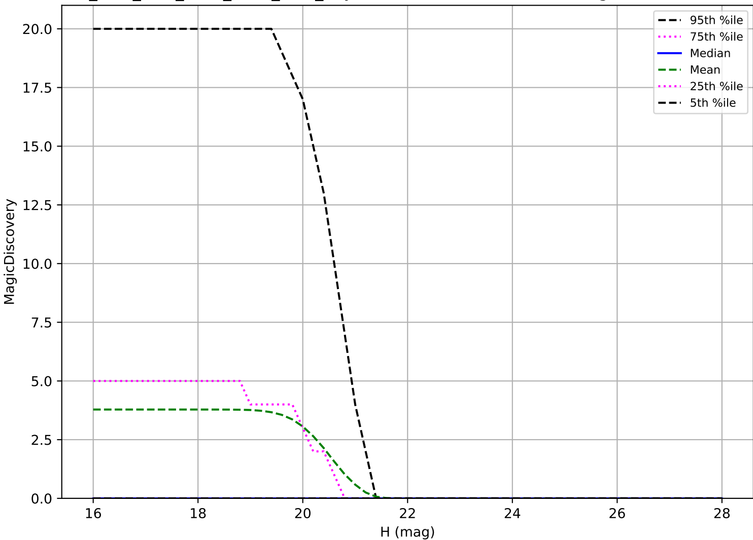
ddf_acor_sf15_lsf30_lsr20_v3.4_10yrs: Vatira 6 detections in 60 nights detection loss
