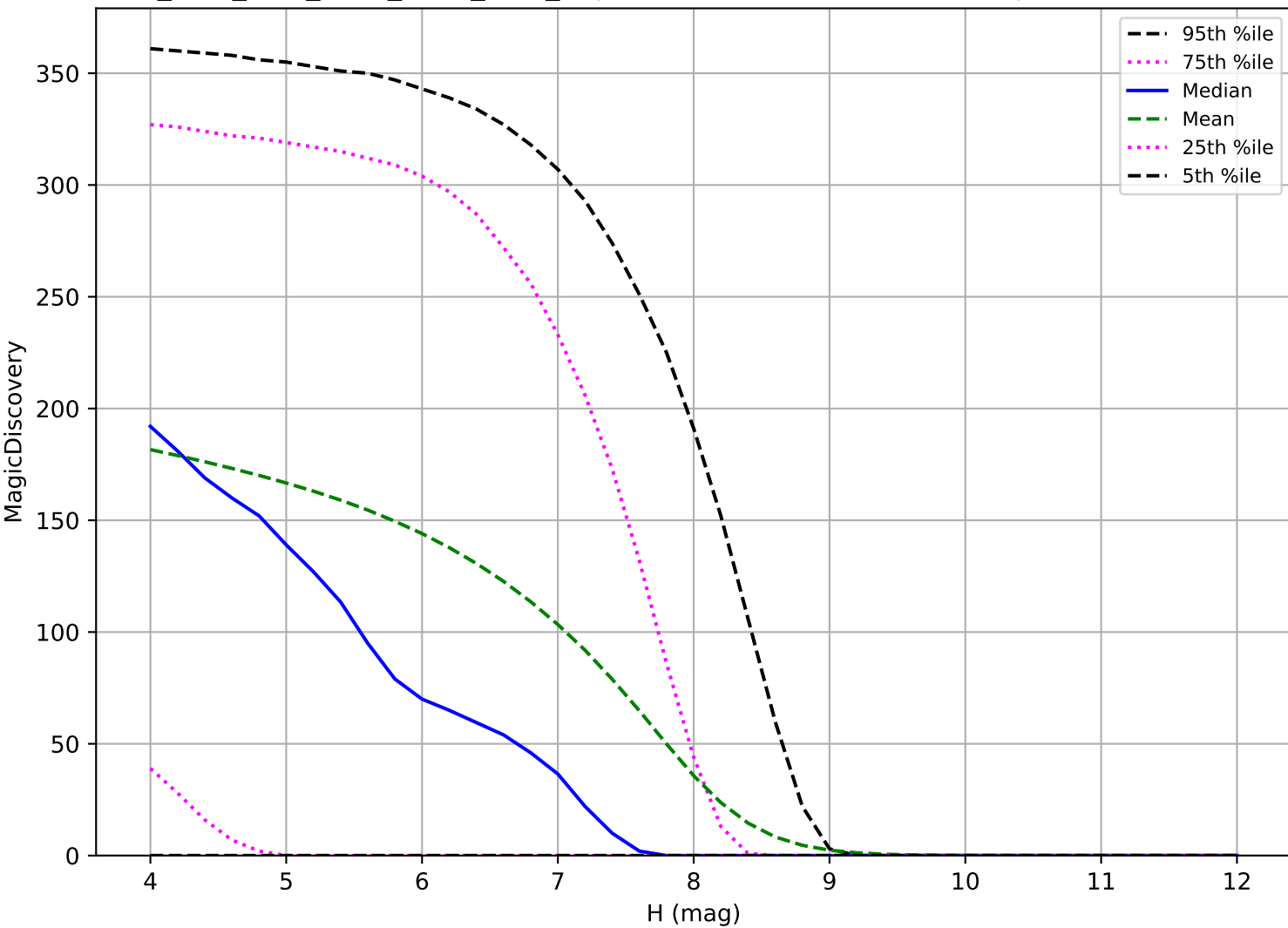
ddf_acor_sf15_lsf30_lsr20_v3.4_10yrs: TNO 6 detections in 60 nights detection loss
