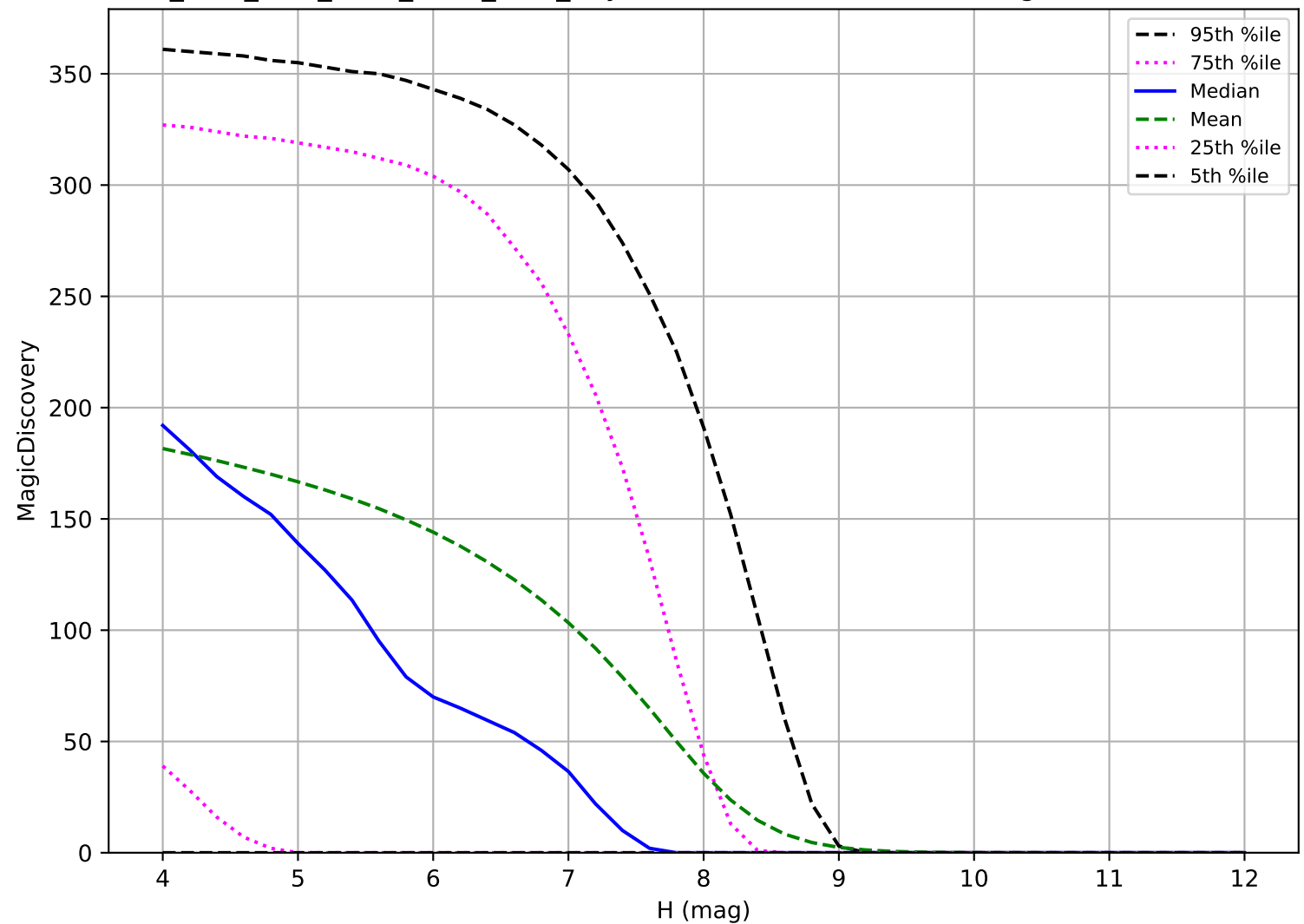
ddf_acor_sf15_lsf30_lsr20_v3.4_10yrs: TNO 6 detections in 60 nights detection loss
