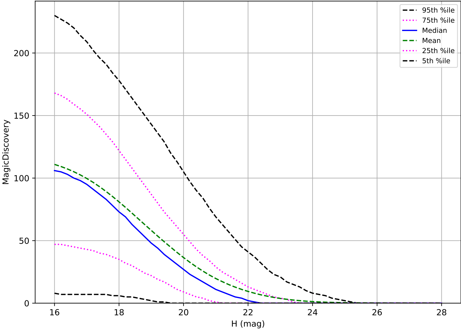
ddf_acor_sf15_lsf30_lsr20_v3.4_10yrs: PHA 6 detections in 60 nights detection loss
