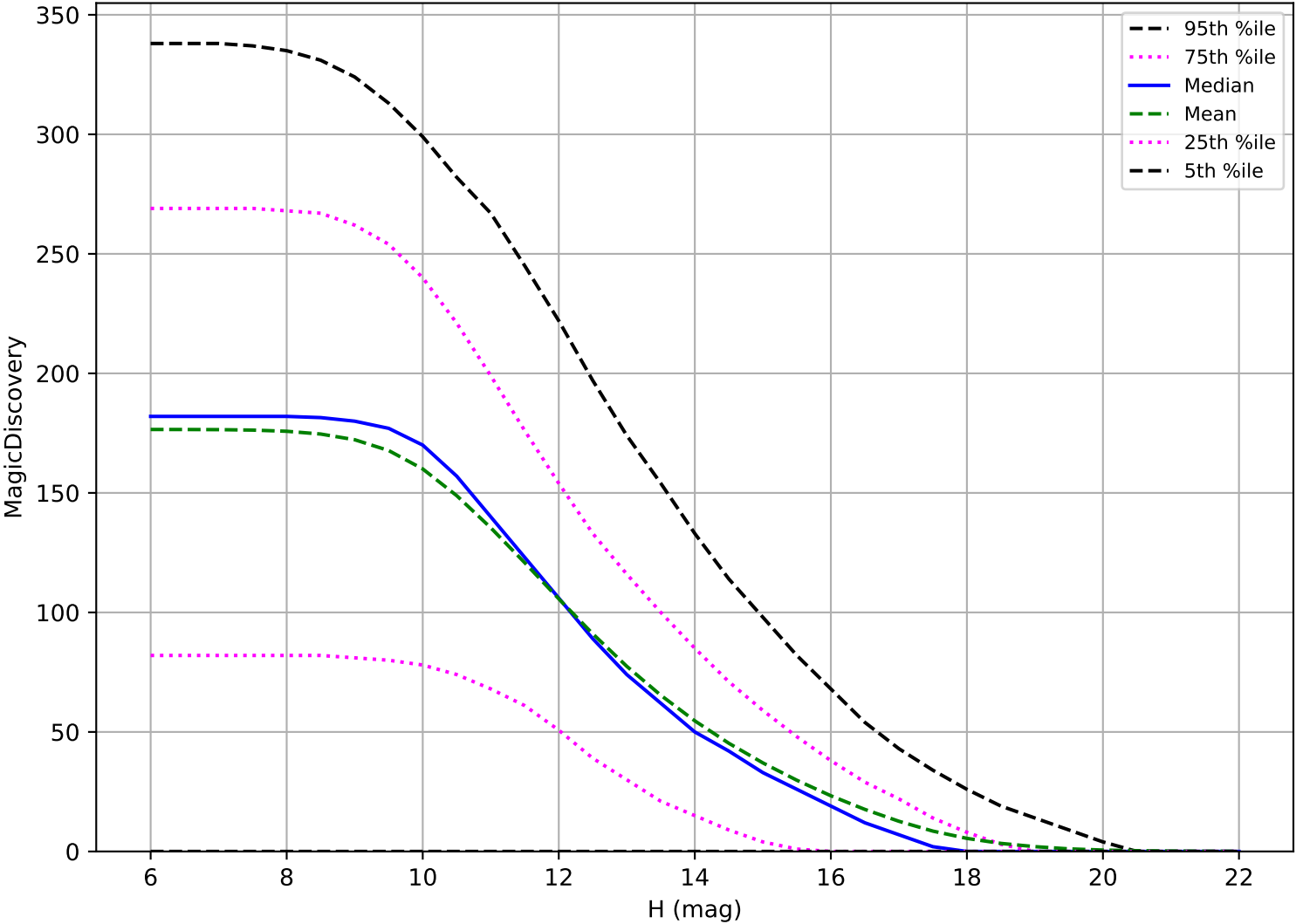
ddf_acor_sf15_lsf30_lsr20_v3.4_10yrs: OCC_r5 6 detections in 60 nights detection loss
