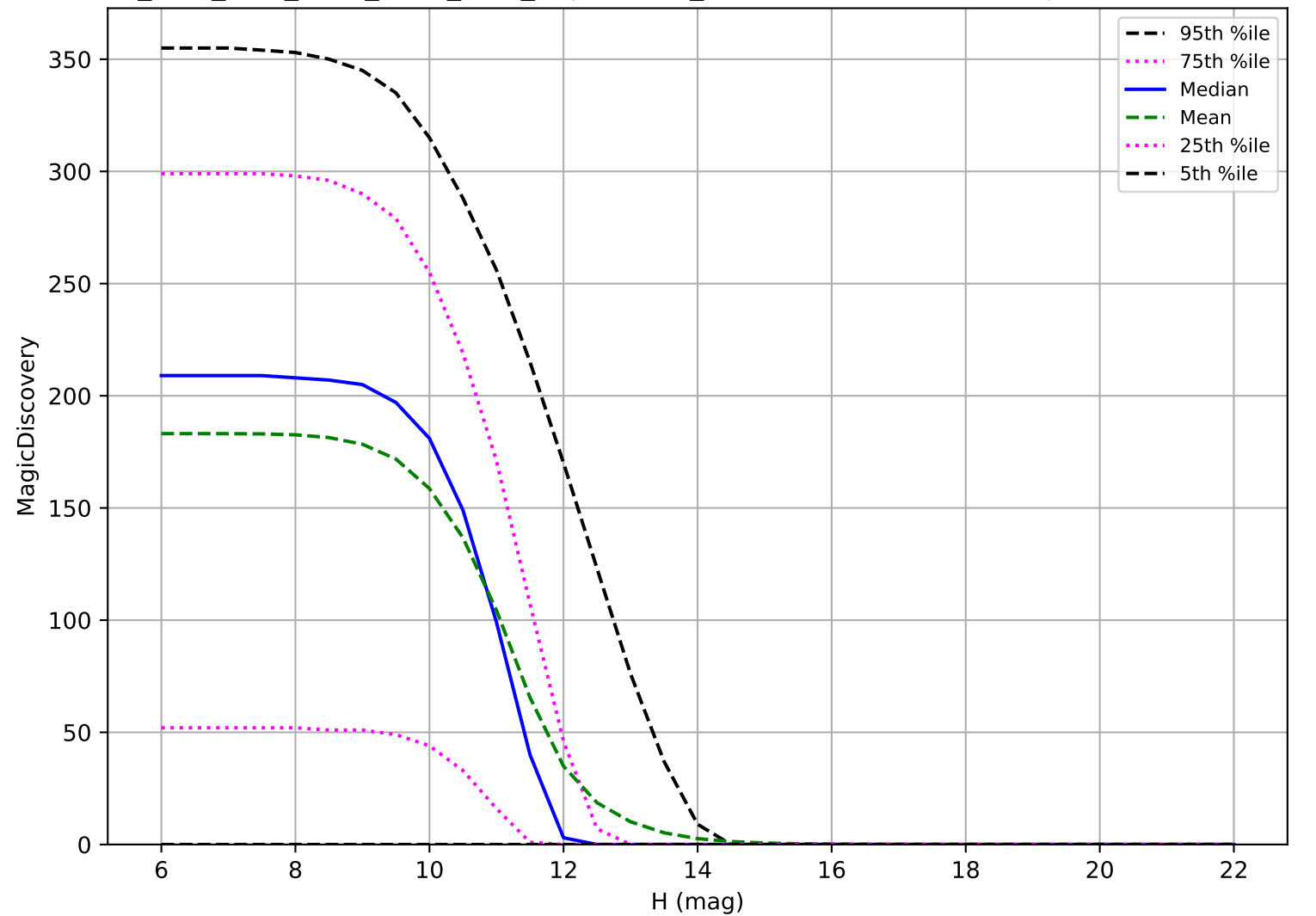
ddf_acor_sf15_lsf30_lsr20_v3.4_10yrs: OCC_r20 6 detections in 60 nights detection loss
