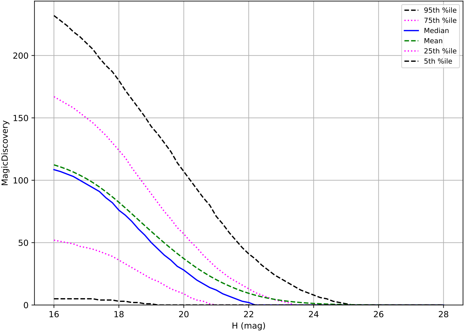
ddf_acor_sf15_lsf30_lsr20_v3.4_10yrs: NEO 6 detections in 60 nights detection loss
