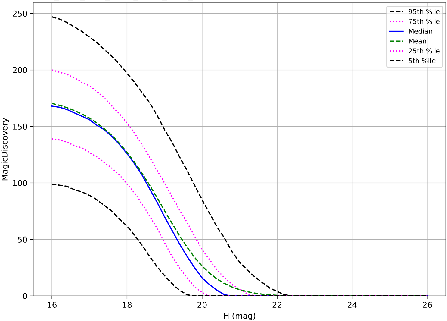
ddf_acor_sf15_lsf30_lsr20_v3.4_10yrs: MBA 6 detections in 60 nights detection loss
