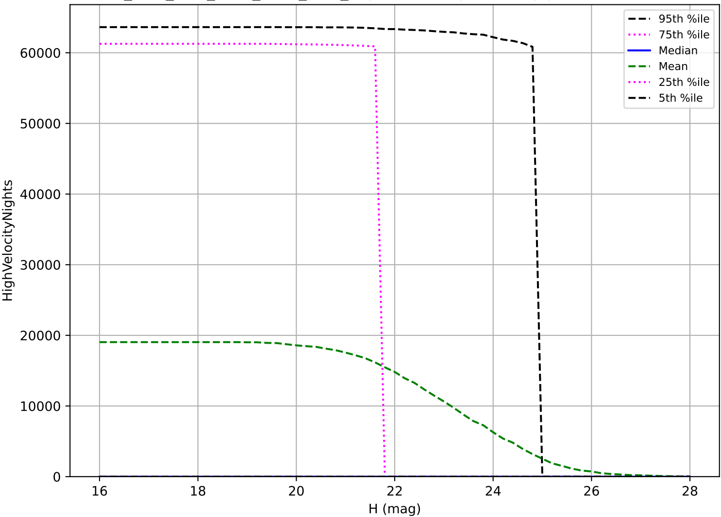
ddf_acor_sf15_lsf30_lsr20_v3.4_10yrs: NEO High velocity pair detection loss
