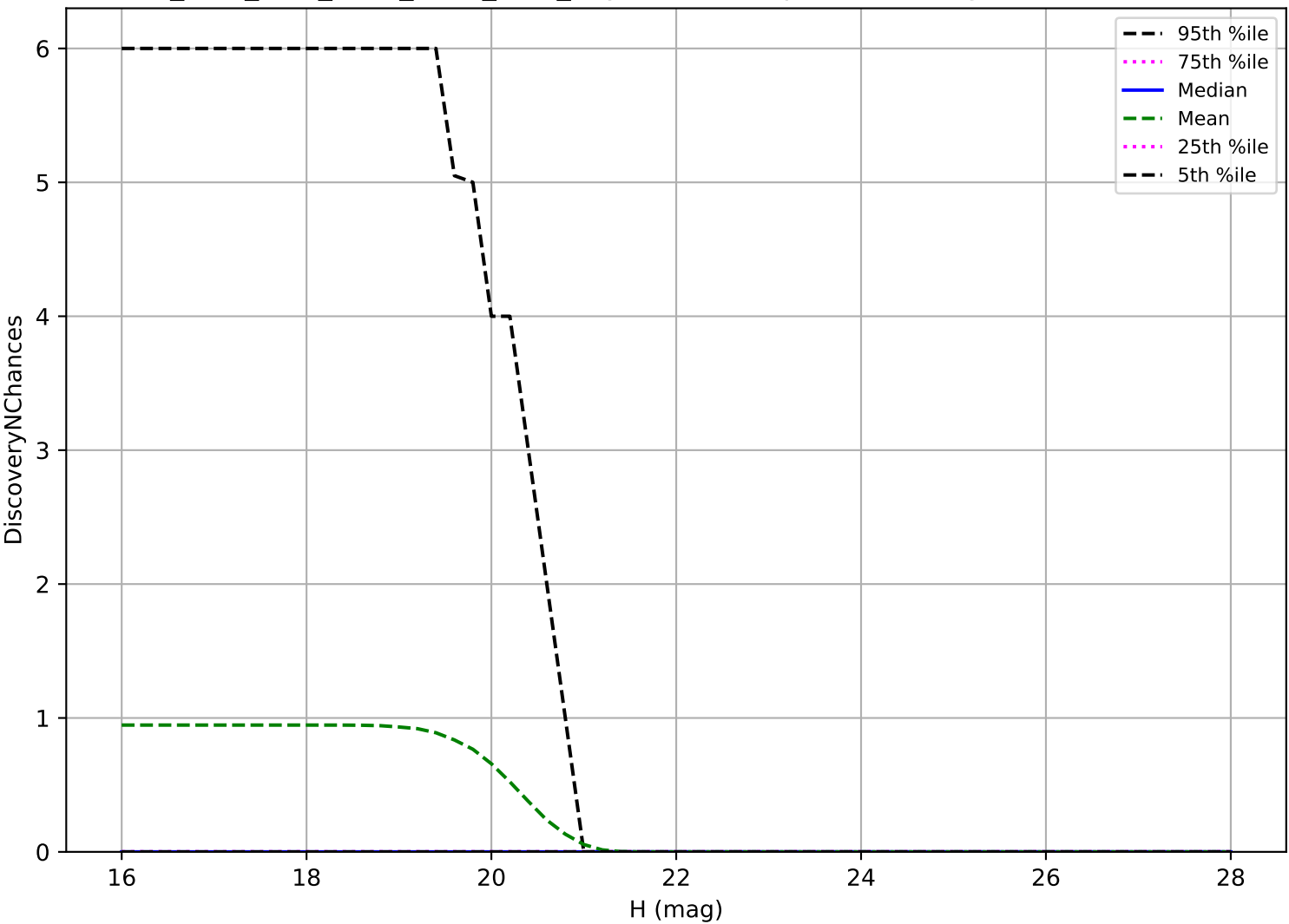
ddf_acor_sf15_lsf30_lsr20_v3.4_10yrs: Vatira 3 pairs in 15 nights detection loss
