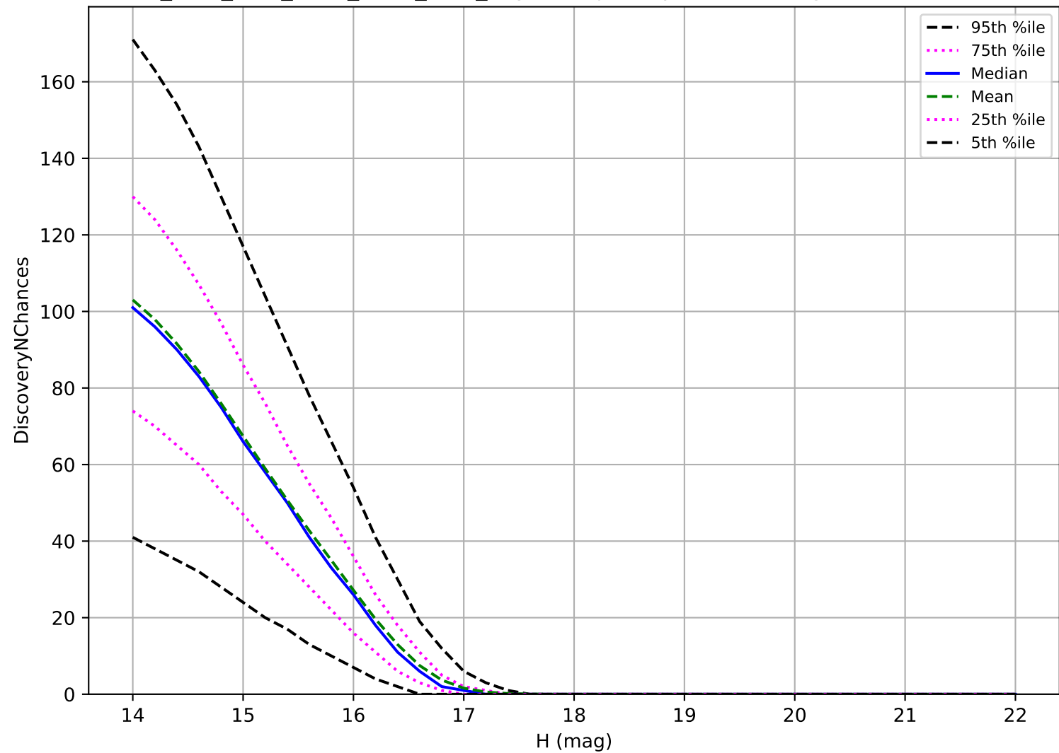
ddf_acor_sf15_lsf30_lsr20_v3.4_10yrs: Trojan 3 pairs in 15 nights detection loss
