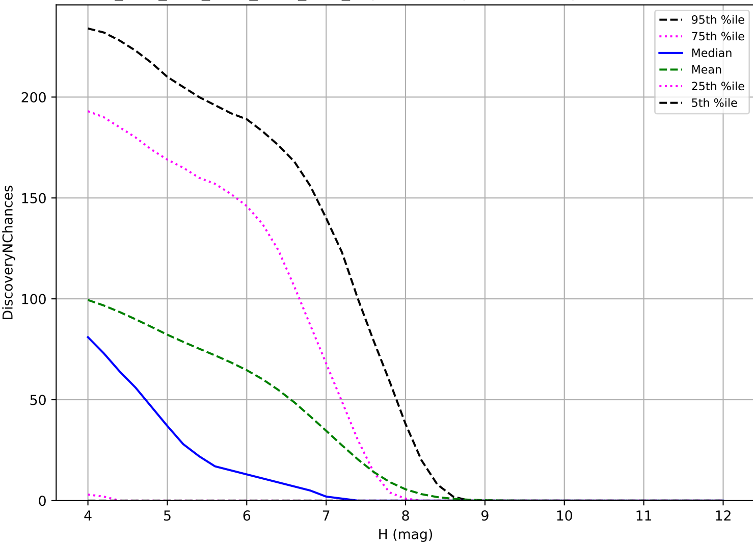
ddf_acor_sf15_lsf30_lsr20_v3.4_10yrs: TNO 3 pairs in 15 nights detection loss
