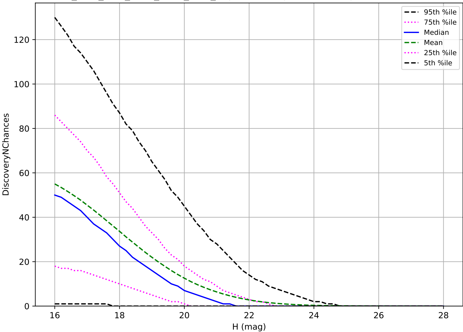
ddf_acor_sf15_lsf30_lsr20_v3.4_10yrs: PHA 3 pairs in 15 nights detection loss
